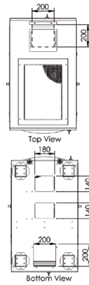
Bottom View
