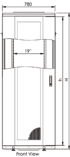
Front View
