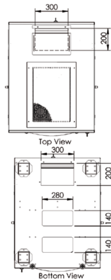
Bottom View
